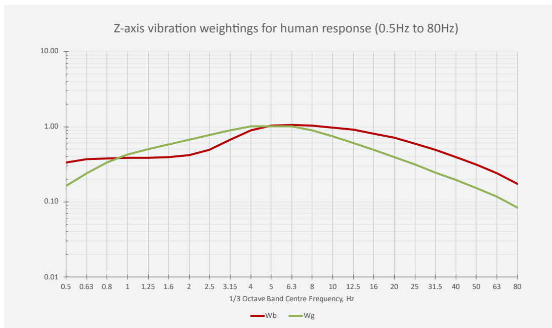
Figure 3: Vibration weightings (reproduced from BS 6472:2008)
